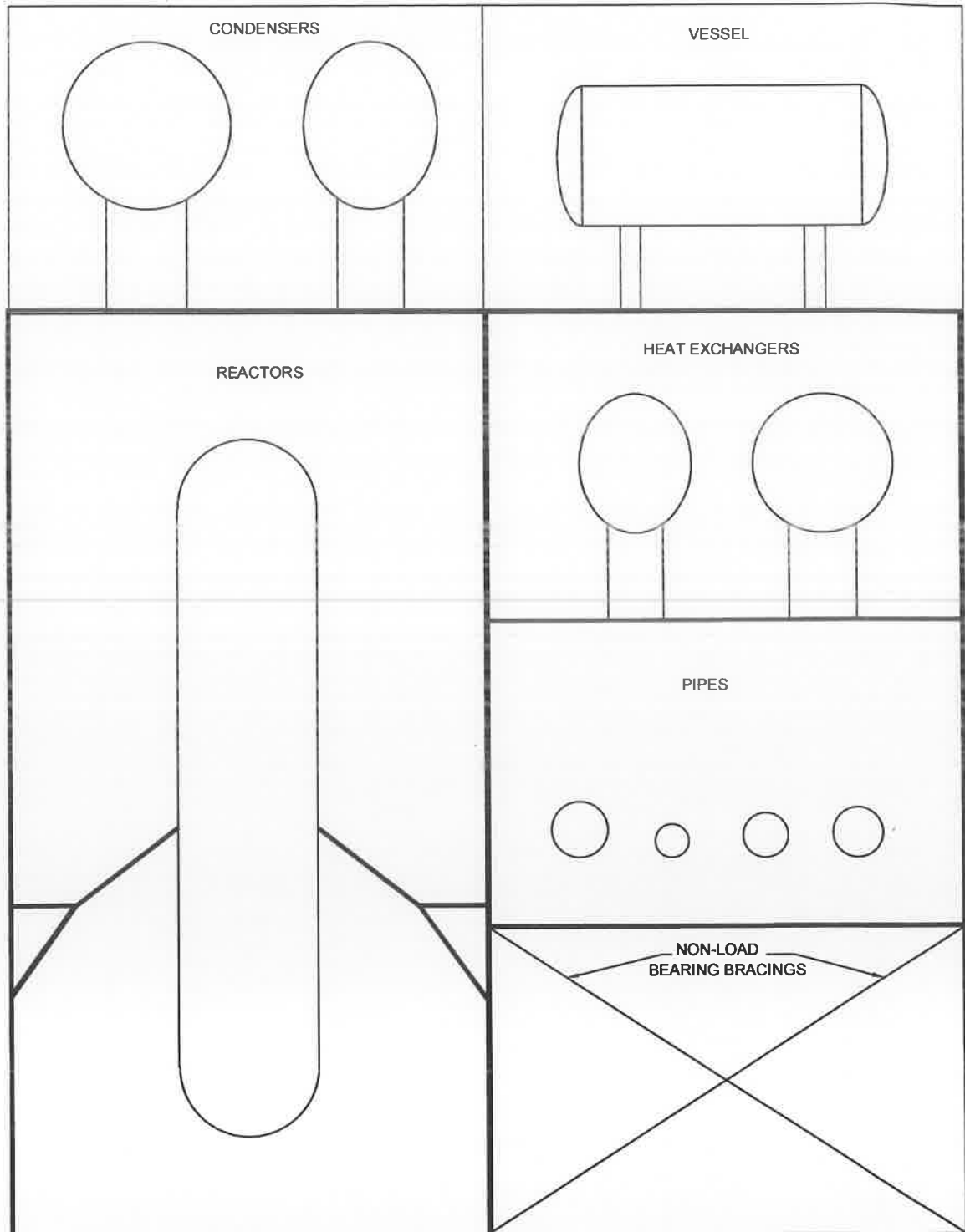
Fig.NO.5.1:- Structures supporting fire potential equipment in a fire exposed area.
